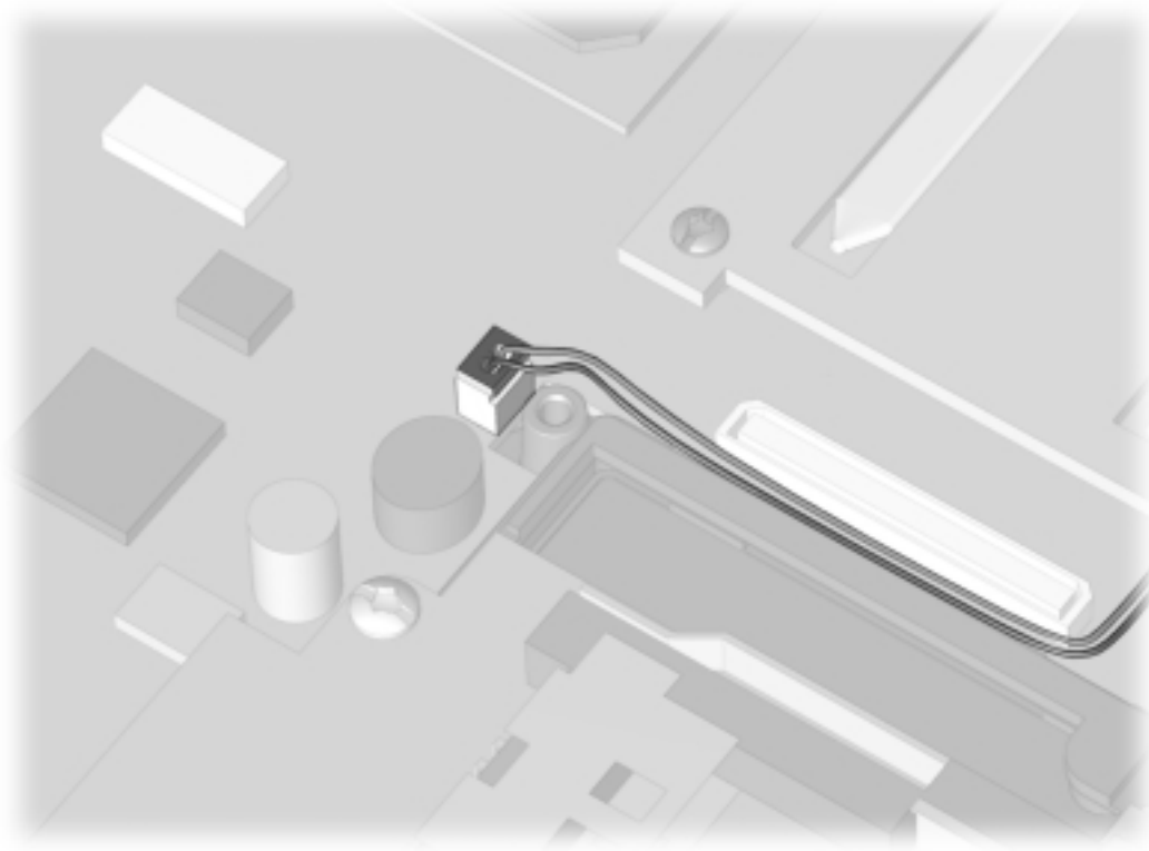
Figure 5-25. Routing the Fan Cable
